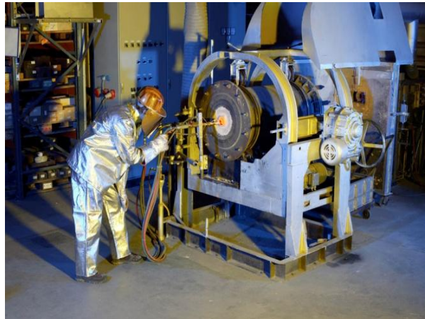
Figure 3-Rotary kiln test
