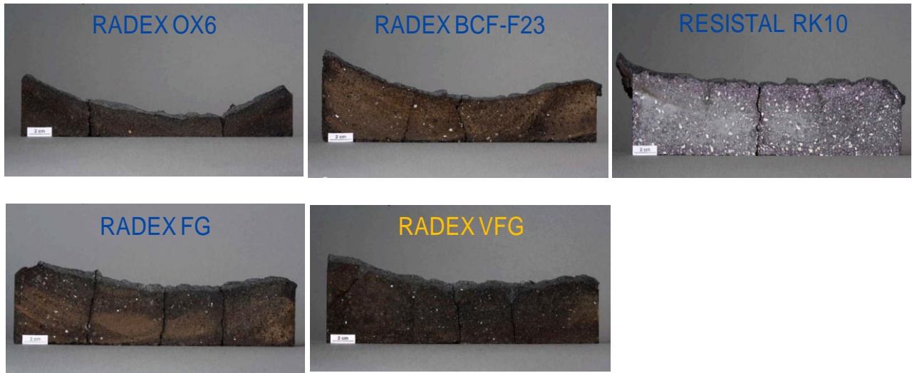
Figure 5-Magnesia-chromite RADEX OX6, RADEX BCF-F23, RADEX FG, RADEX VFG, and alumina-chromia RESISTAL RK10 bricks after the rotary kiln test
