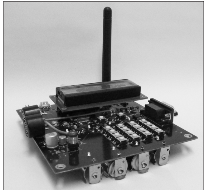
Figure 4. The ultrasonic time-of-flight location tool
