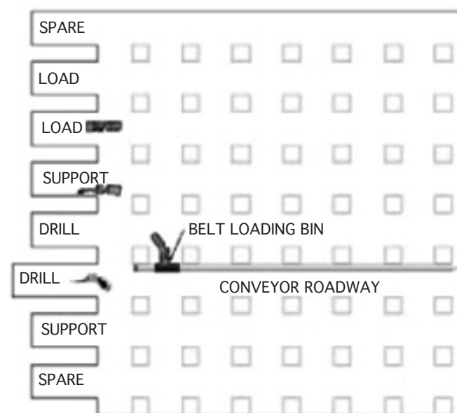
Figure 6. A typical stoping section panel cycle at TRP
