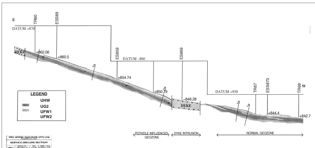
Figure 4. A dip section along part of the on reef service decline, showing the morphology of the reef. Note sections of hangingwall over break where the dip is slightly steeper than average
