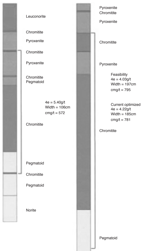
Figure 2. A stratigraphic comparison between the Modikwa Mine cut (left), and TRP mine cut (right). The Modikwa cut is equivalent to the lower UG2 split reef facies in the southern portion of the Two Rivers farm (see Figure 3)
