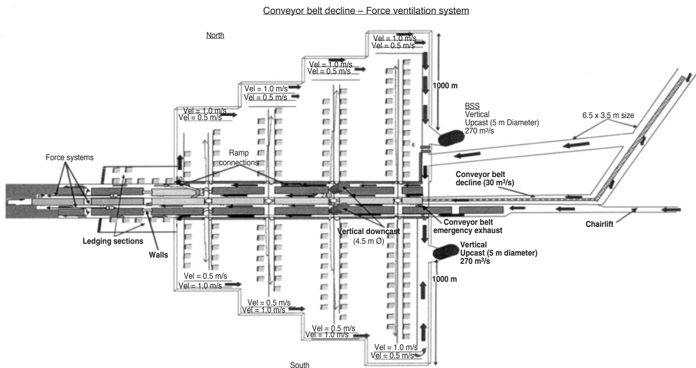
Figure 9. The steady state ventilation design and layout at TRP
