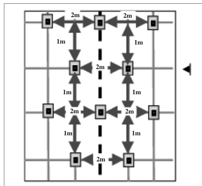
Figure 8. Stope support pattern at Two Rivers Platinum
