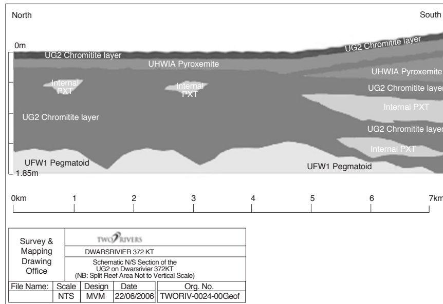
Figure 3. A section N-S of TRP showing the UG2 layer, leaders and pyroxenite partings to the south (after R. Hornsey unpublished 2003)
