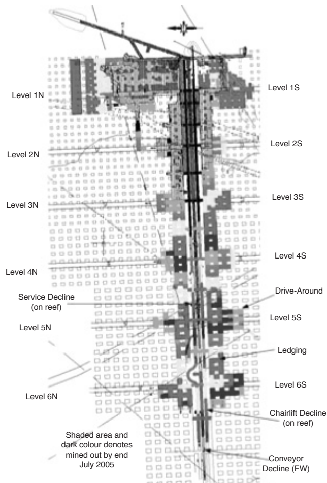
Figure 5. The TRP bord and pillar layout for mechanized mining with the levels down dip and strike roadways
