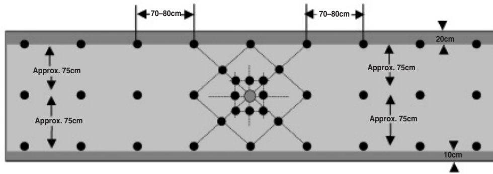
Figure 7. The drill and blast pattern employed in the TRP stope sections
