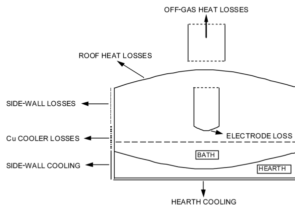
Figure 2. Schematic representation of energy losses around the furnace
