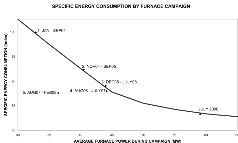
Figure 3. Historical indexed specific energy consumption as a function of furnace power input per campaign (Data for campaign 1 is taken to represent 100%.)
