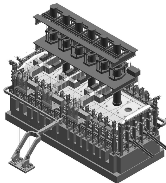
Figure 1. Polokwane smelter furnace
