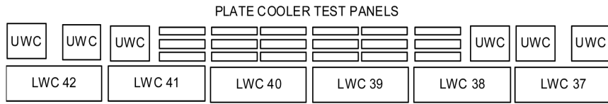
Figure 4. Arrangement of coolers around plate cooler test panel
