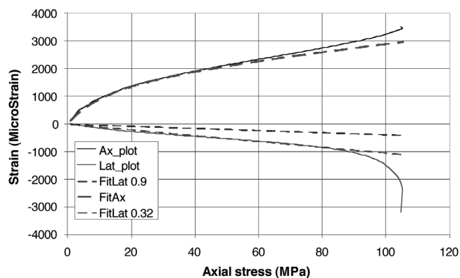
Figure 13. Strain-stress curves from a core extracted from a horizontal borehole (P1b in Figure 2) showing the fitted data determined from Equation 1 with a = 15 and b = 1940 . The lateral plot was fitted using a Poisson's ratio of 0.9 and the plot for a Poisson's ratio of 0.32 is also included for comparison
