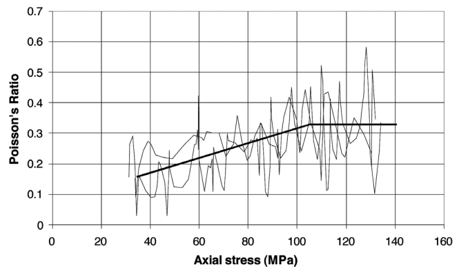
Figure 12. Tangential Poisson's ratio as a function of axial stress, determined under triaxial loading conditions
