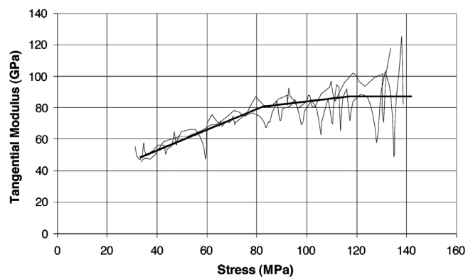
Figure 11. Tangential modulus as a function of axial stress, determined under triaxial loading conditions
