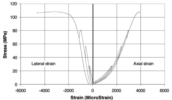
Figure 8. Cycles of loading followed by very slow unloading (KING machine, anorthosite)
