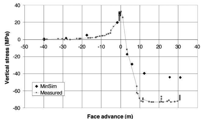
Figure 18. Vertical stress change in response to undermining at position CSIRO2 in Figure 2 compared to an elastic (MinSim) model. Negative face advance refers to the distance of the cell ahead of the face
