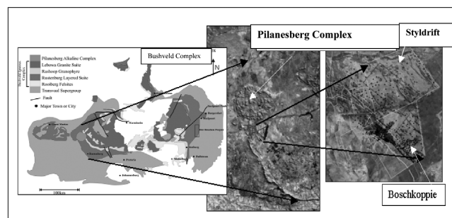
Figure 1. Locality of BRPM within the Bushveld Complex
