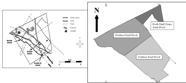
Figure 3. Structural blocks influencing the evaluation of BRPM
