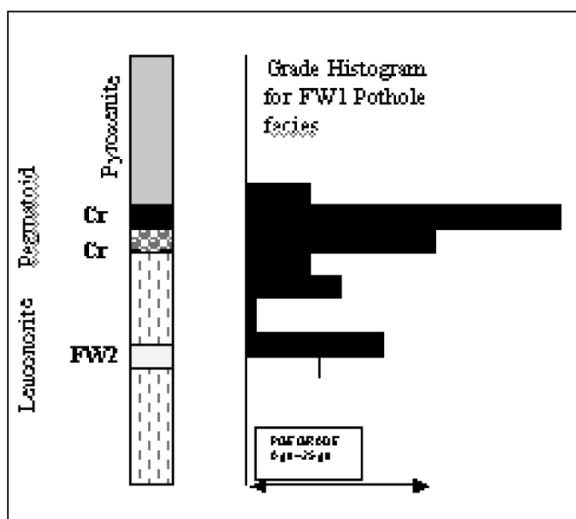
Figure 7. Grade profile of the FW1 pothole facies at 10cm intervals
