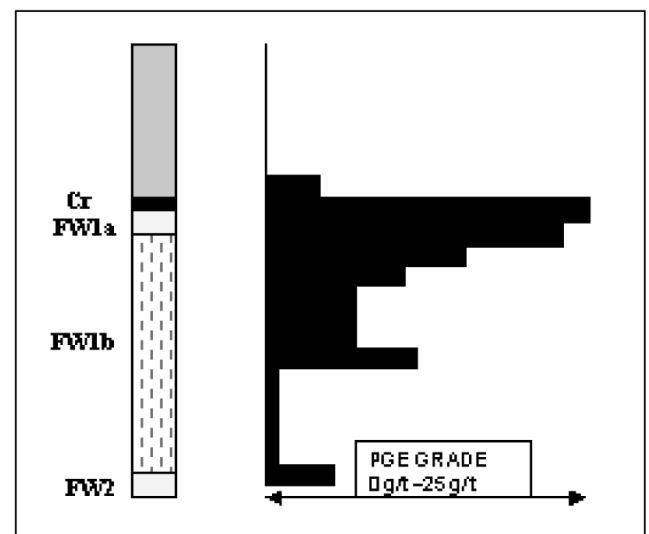
Figure 6. Grade profile of the contact facies at 10cm intervals
