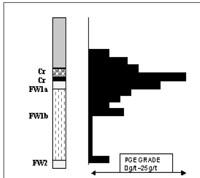
Figure 5. Grade profile of the pegmatoidal facies at 10cm intervals
