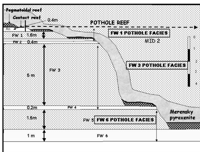
Figure 4. Facies distribution at BRPM
